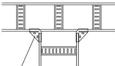
90 DEG ANGLE PIECE BRACKET PART NUMBER : # APB 01
